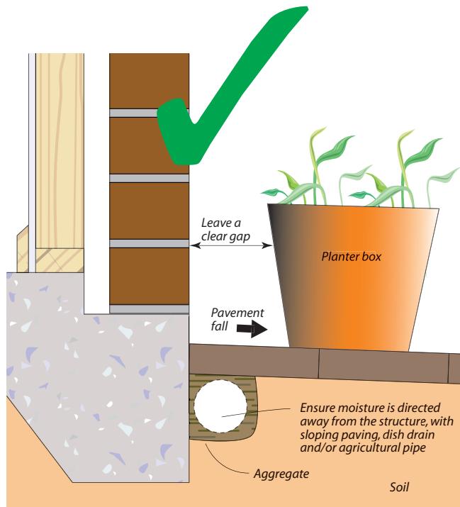
Fig 11: Treatment of paving and planter boxes
